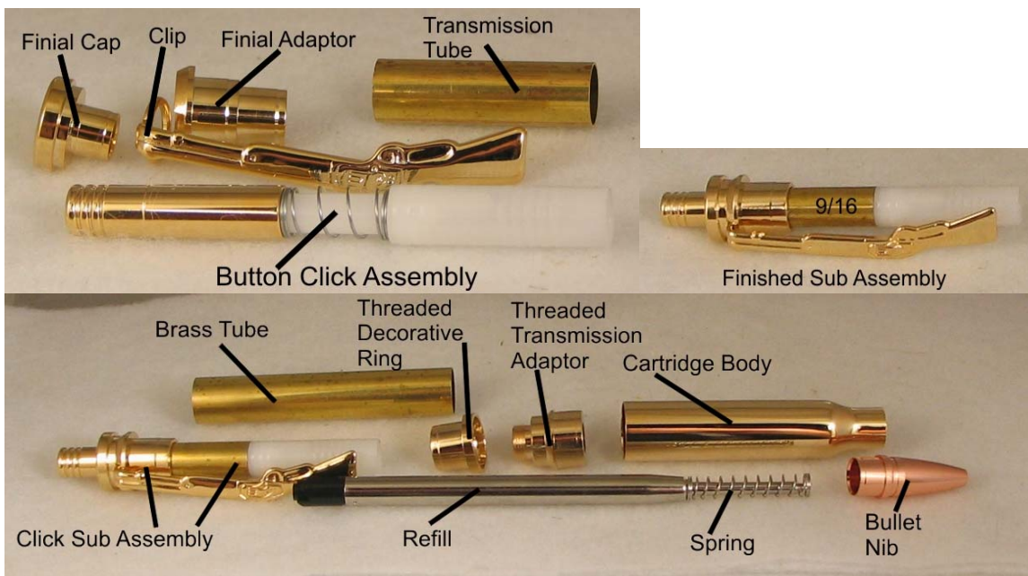
Parts Diagram
